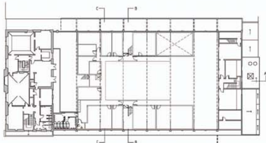
First Floor Plan (Phase 3) N.T.S.
