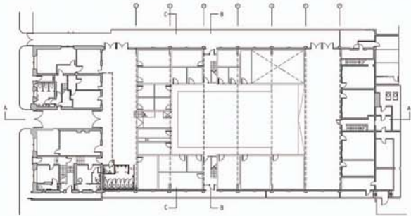
Ground Floor Plan (Phase 2) N.T.S.
