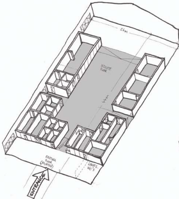
Phase 2-Internal Layout
